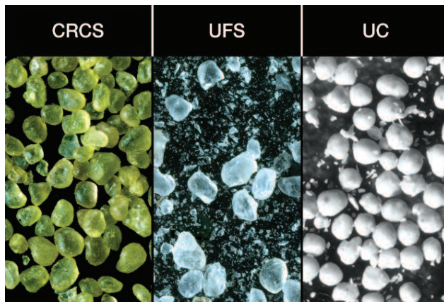
Different proppant types - CRCS, UFS and UC - are shown after being tested with the wet hot crush test at 8,000 psi. (Images courtesy of Momentive Specialty Chemicals Inc.)
